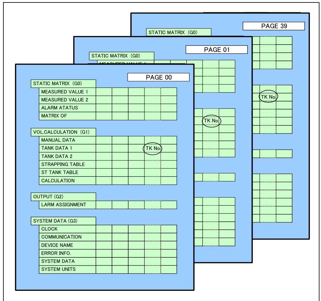
Fig. 18 Database structure
