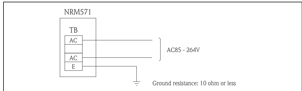
Fig 6. Power Supply
