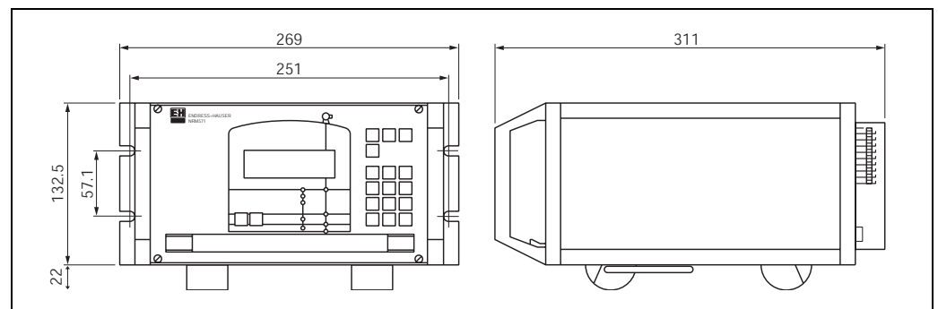
Fig 2. NRM dimension
