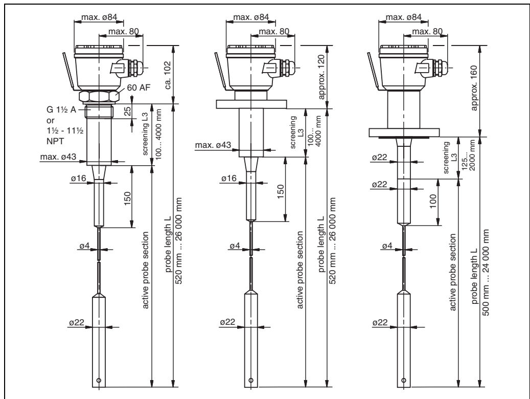
From left to right: Multicap DC 21 with threaded boss and uninsulated metallic screening Multicap DC 21 with flange and uninsulated metallic screening Multicap DC 21 with PTFE-clad flange and fully insulated screening
