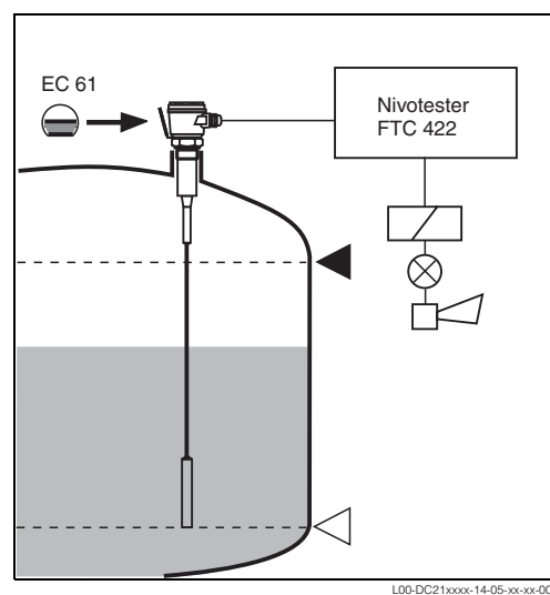
Two-point control
