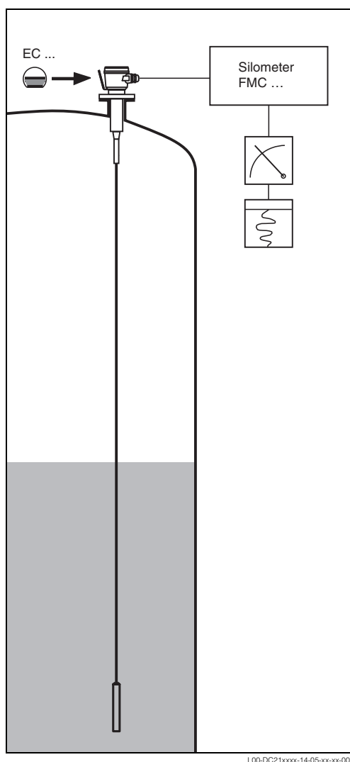
Continuous measurement, e.g. using probe with screening against condensation in the nozzle
