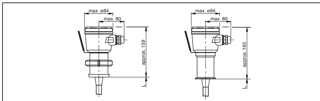
left: Multicap DC 21 with sanitary thread DIN 11851-DN 50 right: Multicap DC 21 with 2" Triclamp coupling
