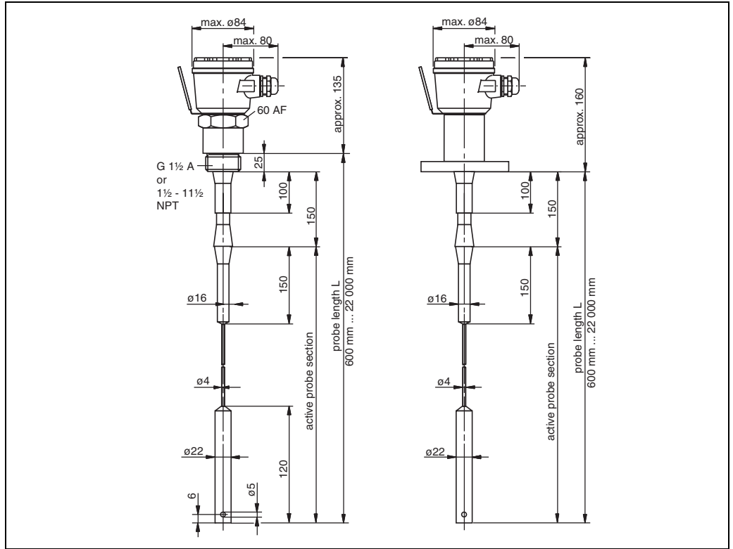
From left to right: Multicap DC 21 with threaded boss and active build-up compensation Multicap DC 21 with flange and active build-up compensation
