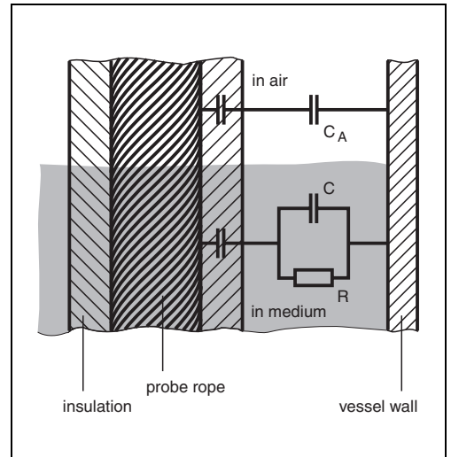
Equivalent circuit for capacitance measurement with fully insulated probes
