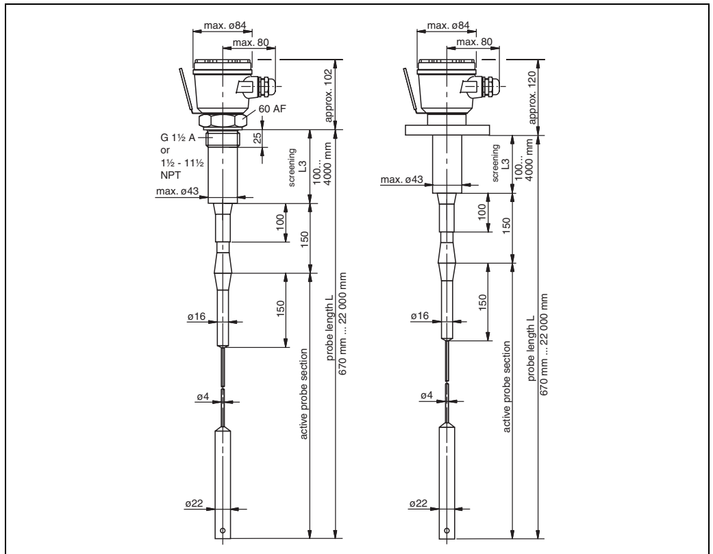
From left to right: Multicap DC 21 with threaded boss, screening and active build-up compensation Multicap DC 21 with flange, screening and active build-up compensation
