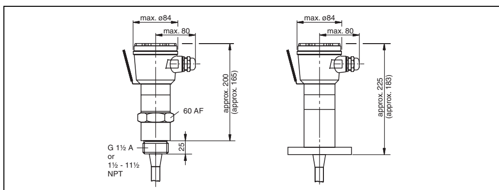
left: Multicap DC 21 with threaded boss and temperature spacer right: Multicap DC 21 with flange and temperature spacer
