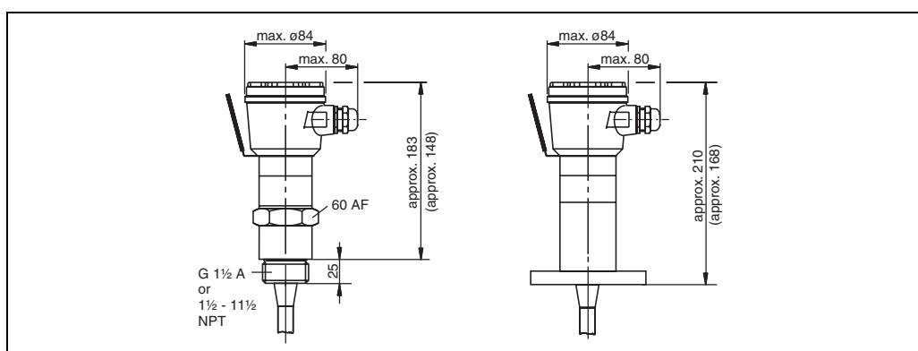
left: Multicap DC 21 with threaded boss and gas-tight gland right: Multicap DC 21 with flange and gas-tight gland
