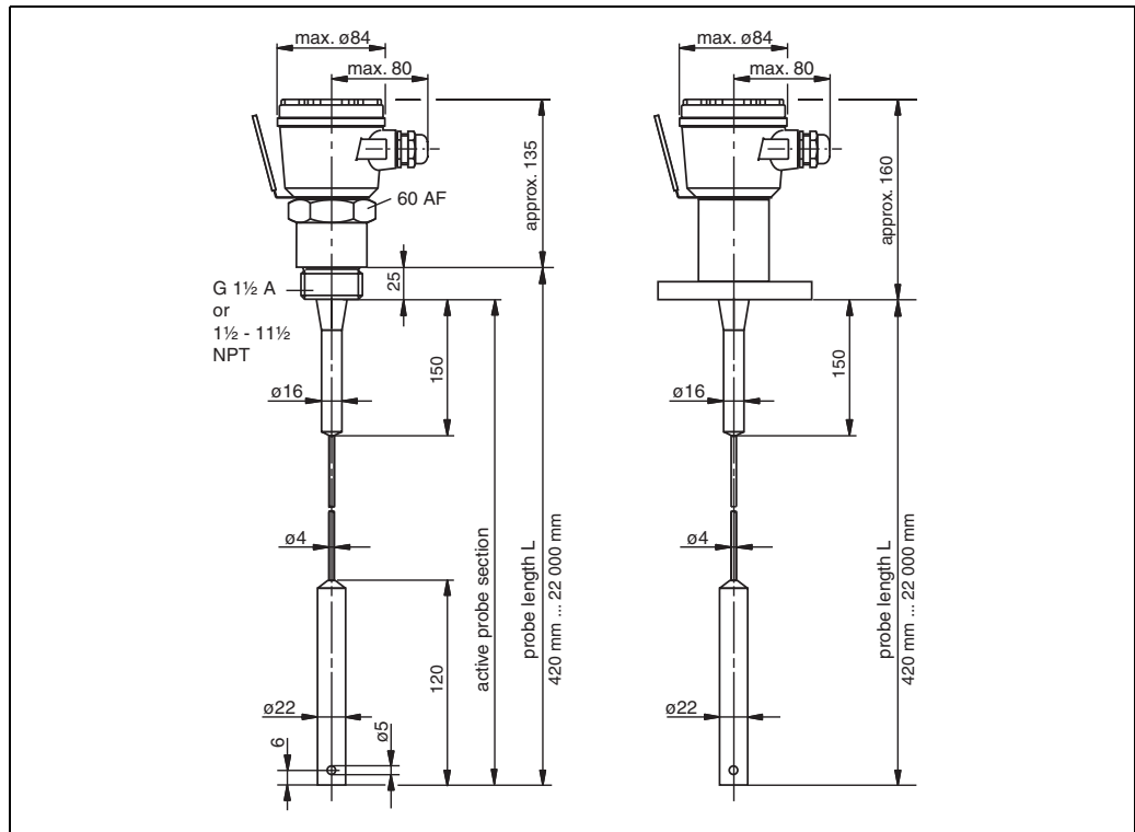
From left to right: Multicap DC 21 with threaded boss Multicap DC 21 with flange
