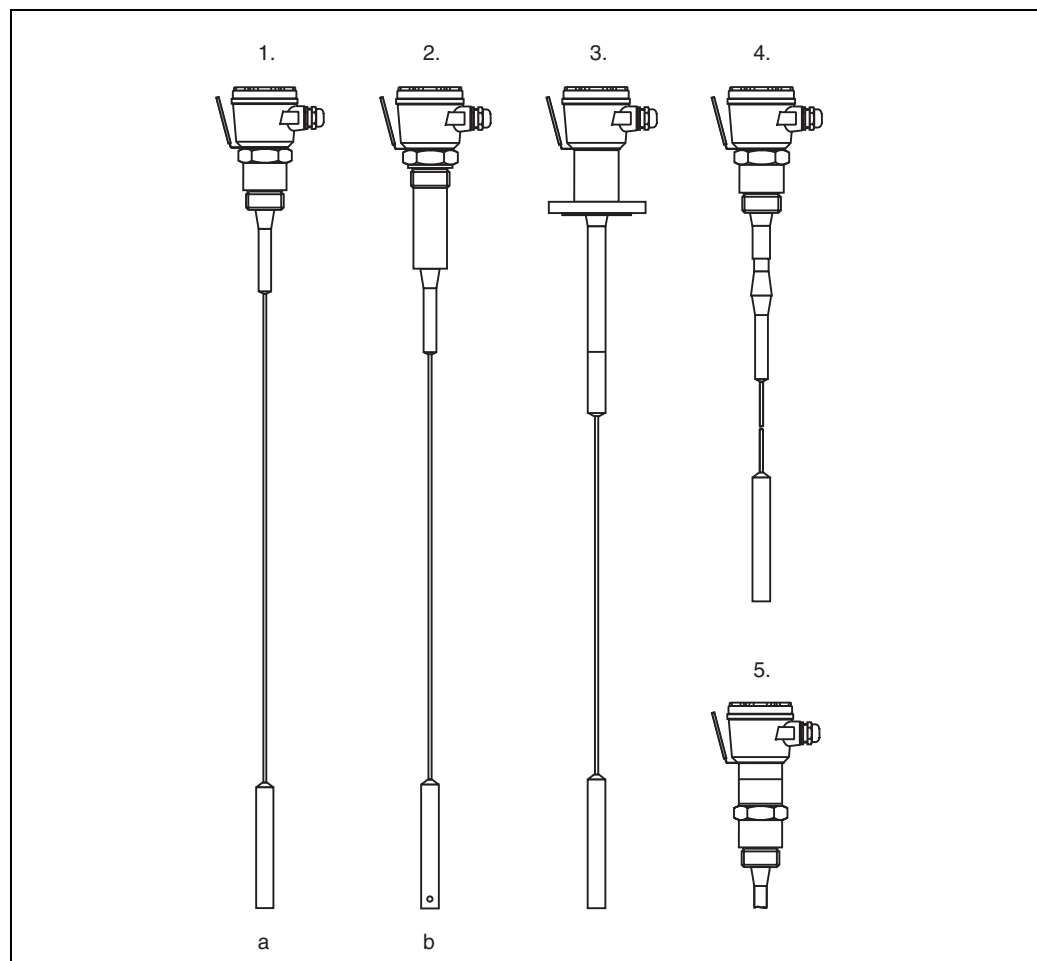
Fully insulated rope probe versions a) Tensioning weight b) Anchor weight with insulated bore
