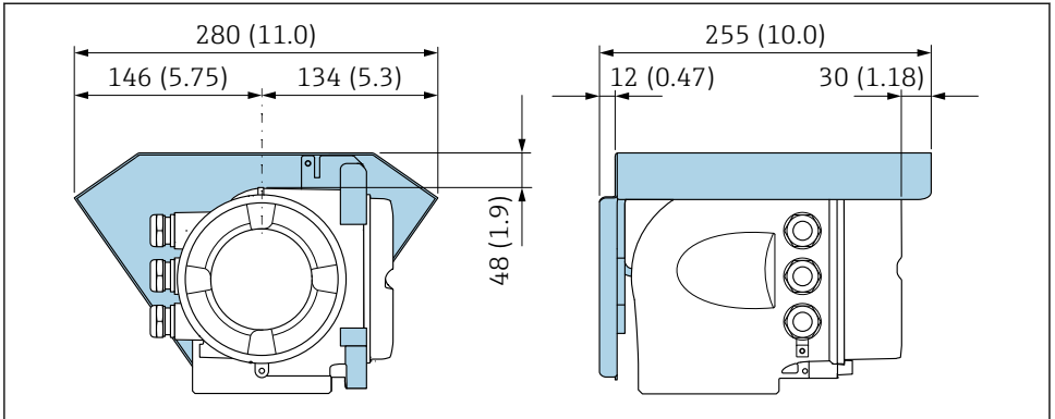
5 Weather protection cover for Proline 500
