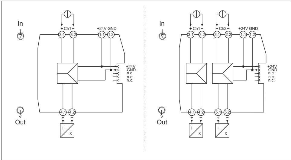
4 Terminal assignment of RNO22: 1-channel version (left), 2-channel version (right)
