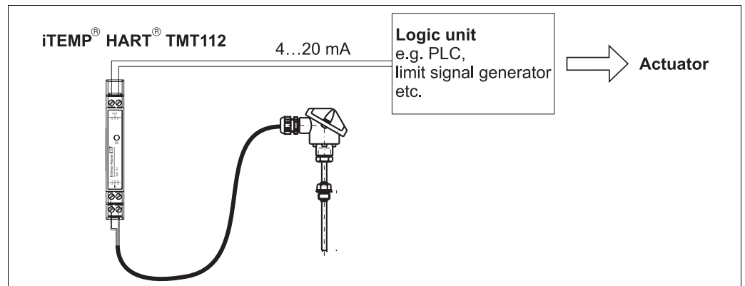
Fig. 2: Safety function (e.g. for limit temperature monitoring) with TMT112 as sub-system
