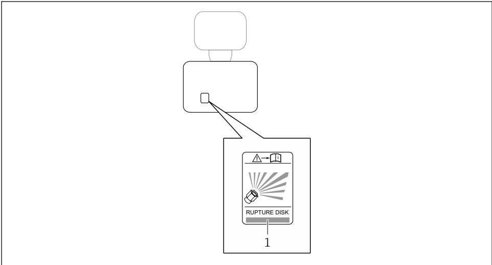
1 Rupture disk label
