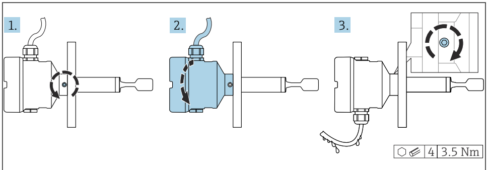
11 Housing with external locking screw and drip loop
