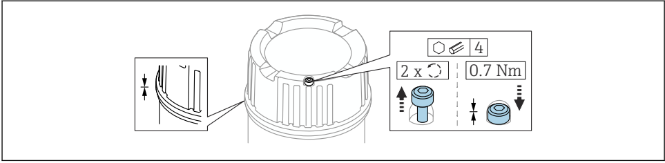
12 Cover with securing screw
