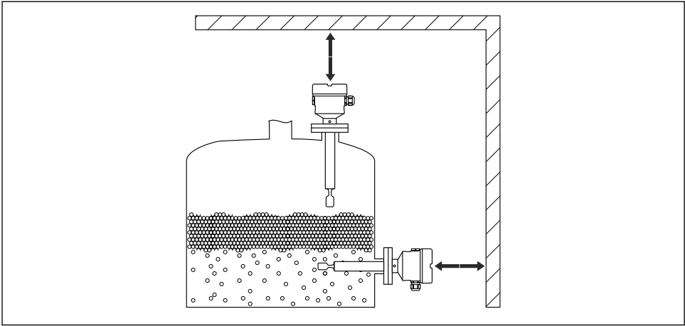
7 Take clearance outside the tank into consideration
