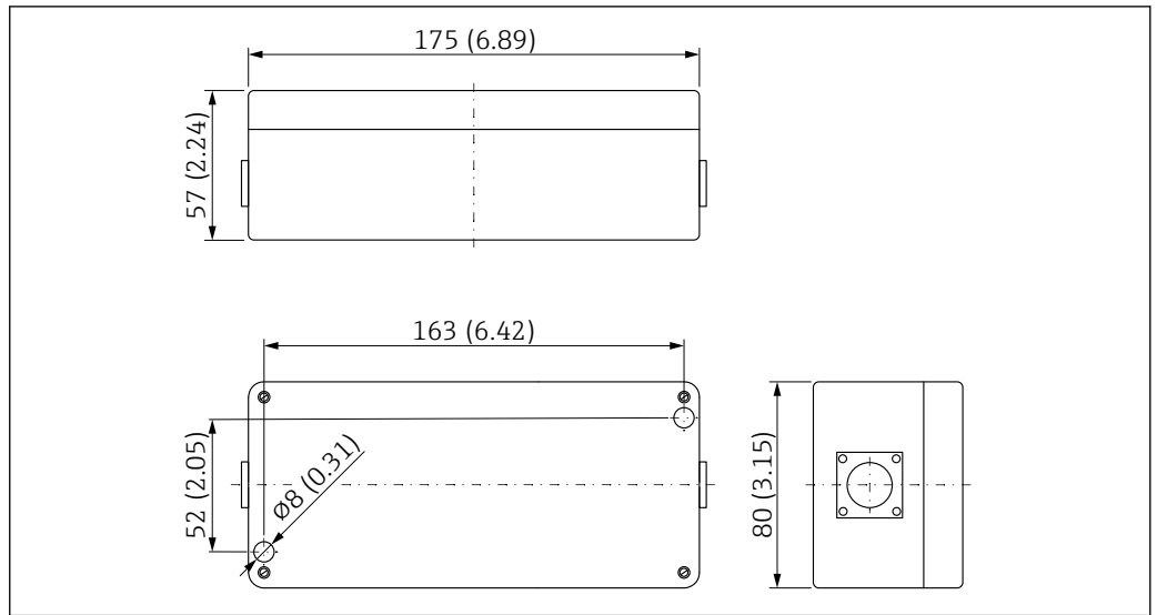
8 Dimensions of housing for remote electronics module. Unit of measurement mm (in)
