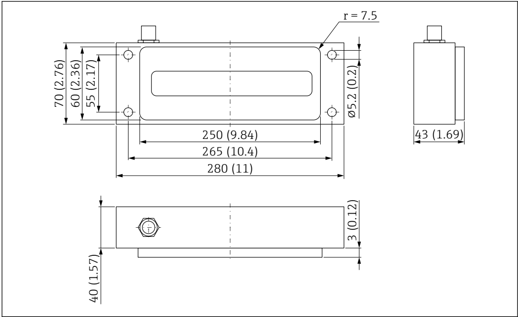
7 Device dimensions. Unit of measurement mm (in)
