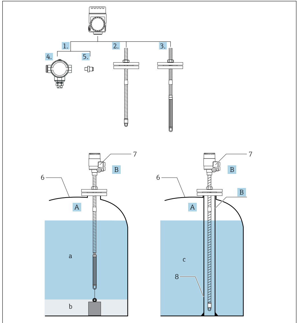
1 NMT539 installation
