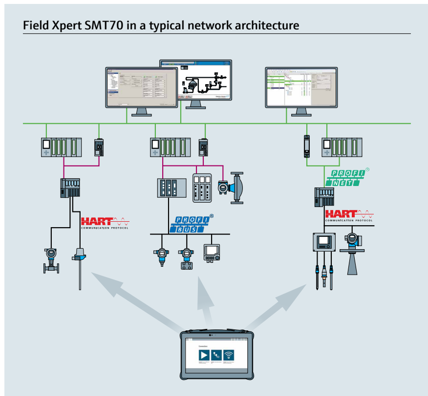
Field Xpert SMT70 as mobile workstation right in the field
