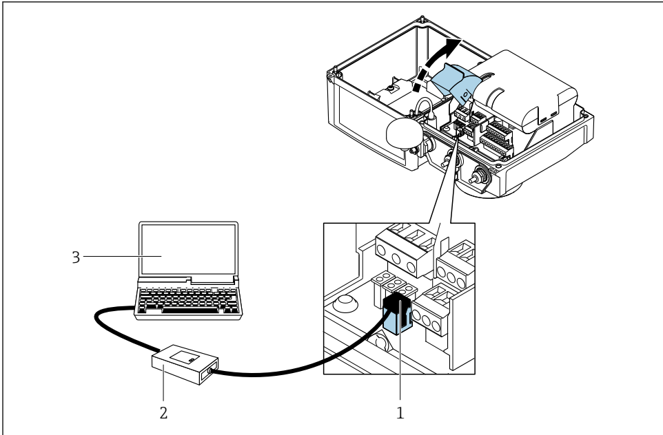
1 Connecting the laptop to the service interface via Commubox FXA291
